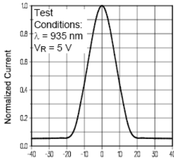
Light Current vs. Angular Displacement
