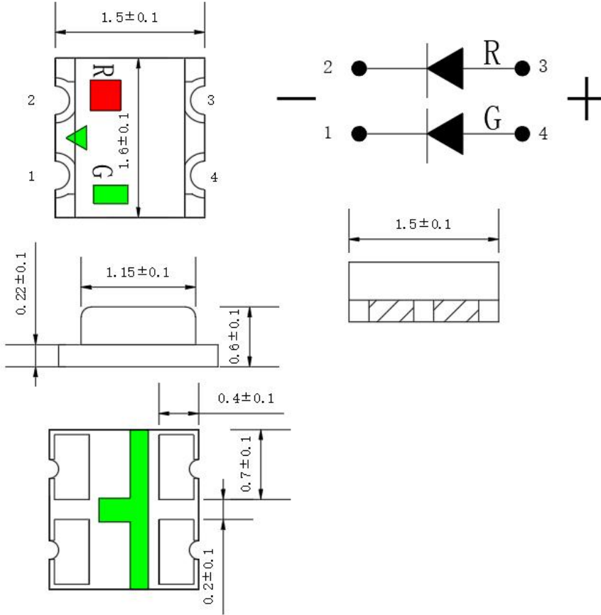
Recommended Solder Pad Design 推荐焊盘设计
