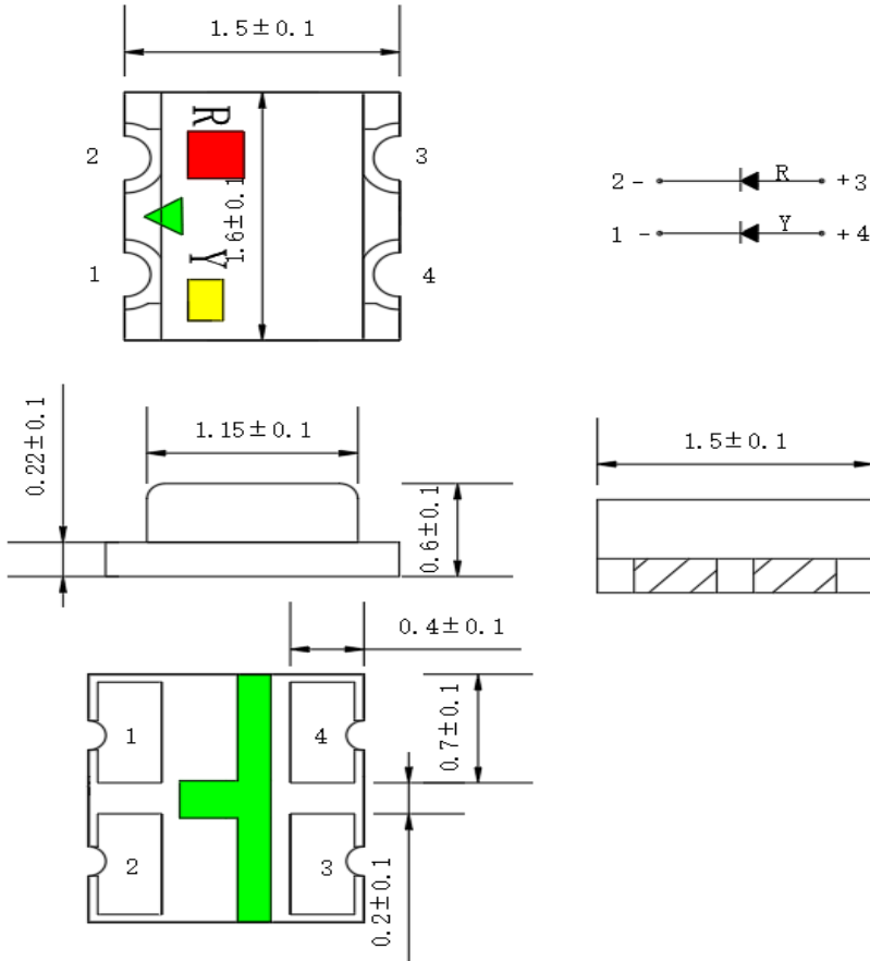
Recommended Solder Pad Design 推荐焊盘设计
