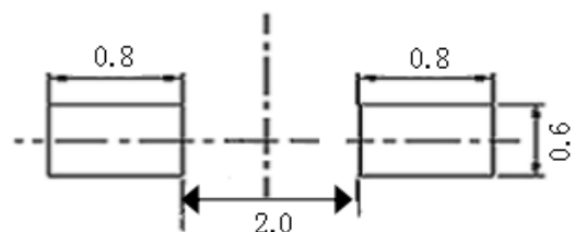
Recommended Soldering Pattern (Units : mm)-
