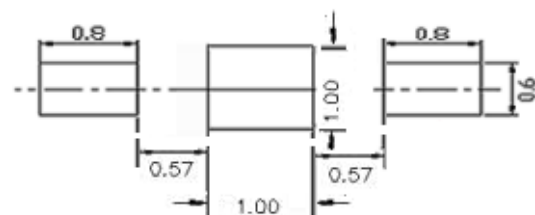
Recommended Soldering Pattern (Units : mm)
