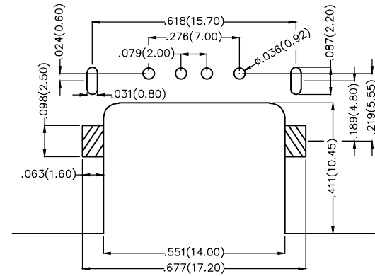
Recommended P.C.Board Layout (General Tolerance : ±.002(0.05))
