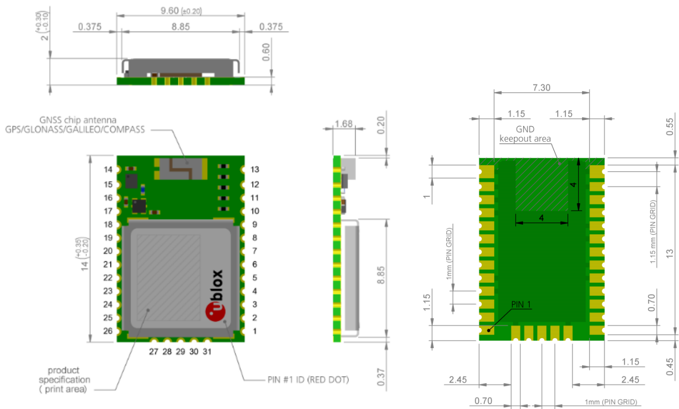
Figure 4: Dimensions (unit: mm)
