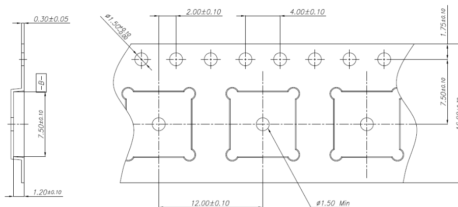
Figure 5: Orientation of EVA-M8M/Q modules on the tape
