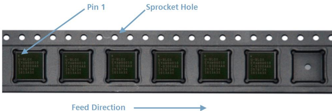
Figure 5: Orientation of EVA-M8M/Q modules on the tape
