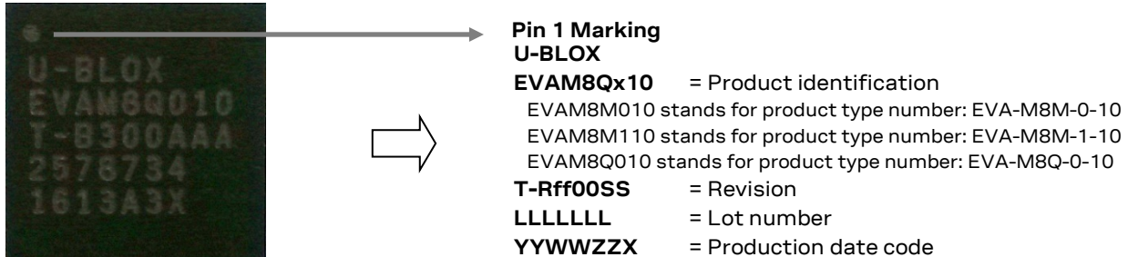
Figure 7: Description of EVA-M8Q product label
