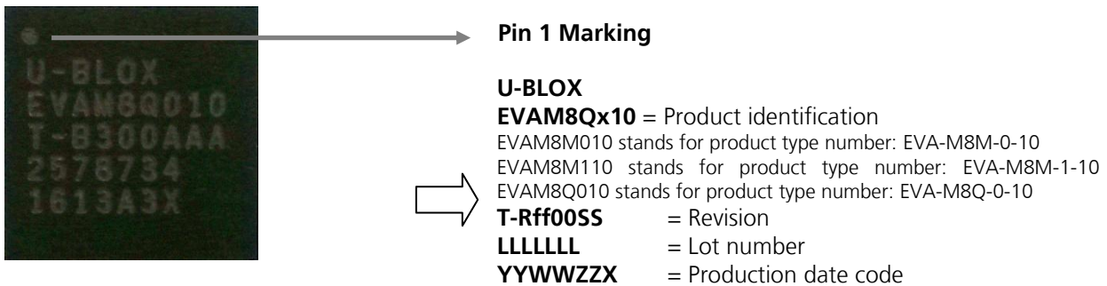
Figure 7: Description of EVA-M8Q product label
