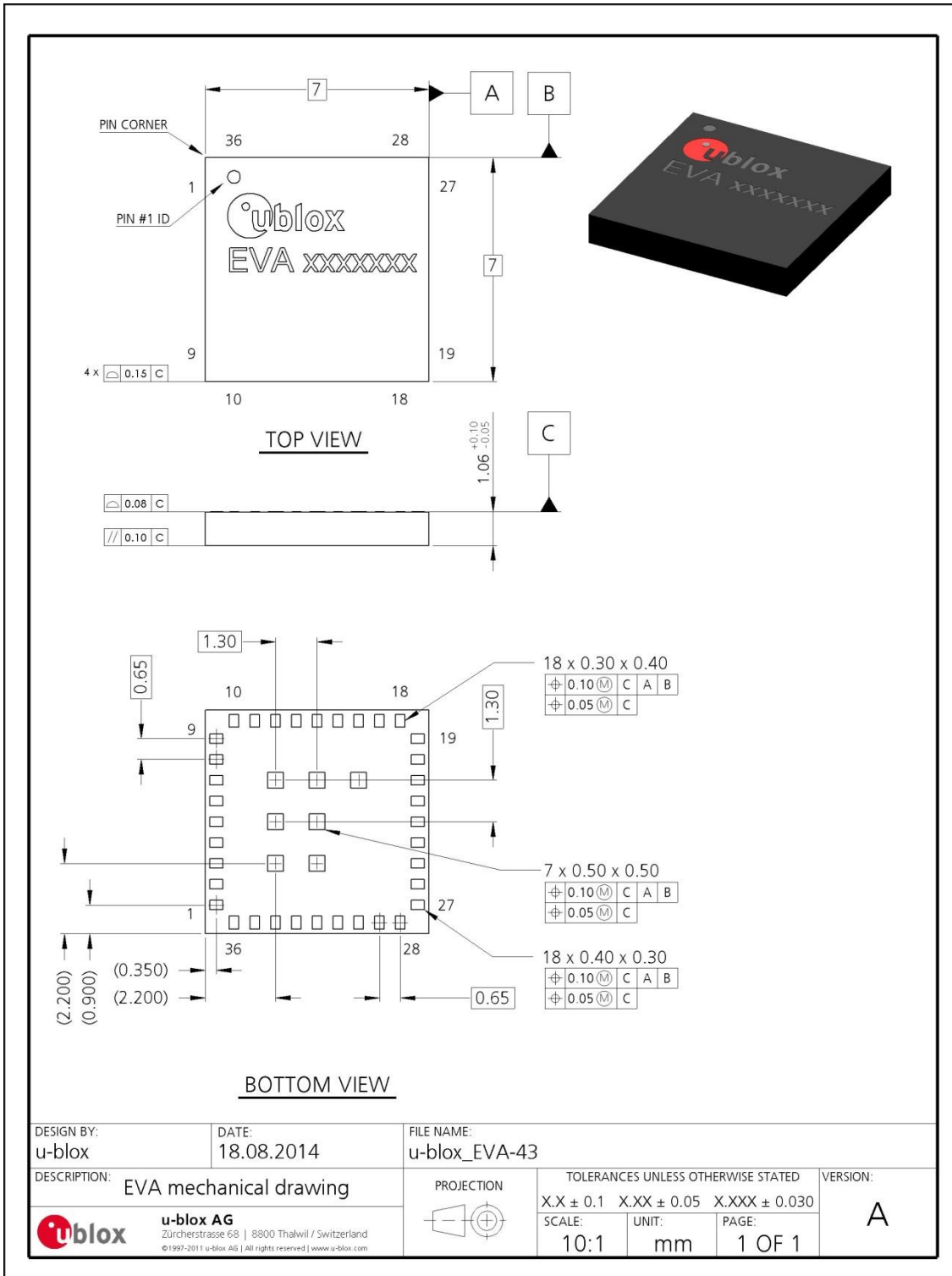
Figure 4: Mechanical drawing for EVA-M8M/Q (LGA43)
