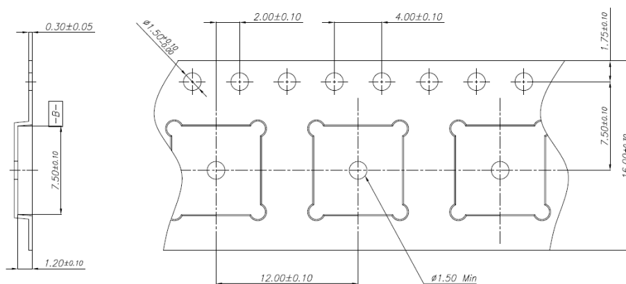
Figure 5: Orientation of EVA-M8Q modules on the tape
