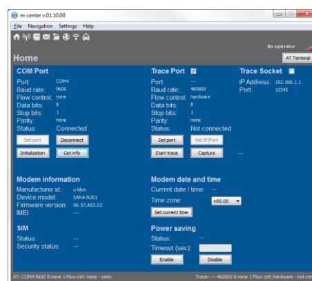
Figure 3: "Home" page
