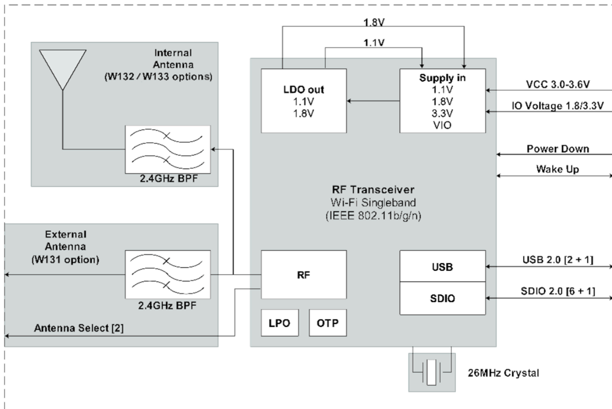
Figure 1: Block diagram of LILY-W1
