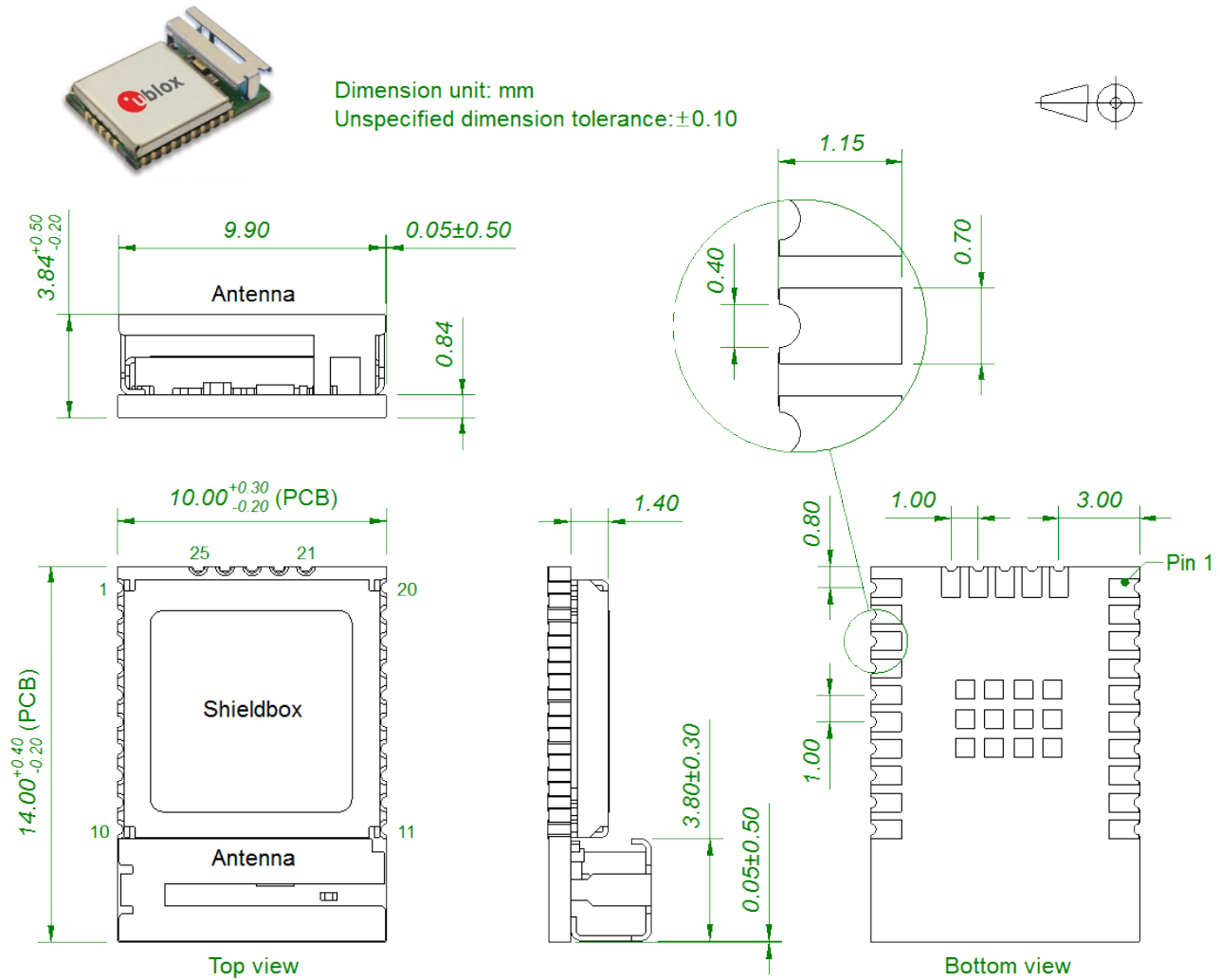
Figure 5: LILY-W132 and LILY-W133 dimensions
