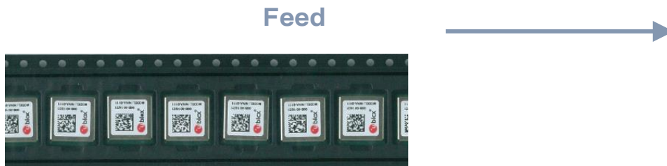
Figure 9: Orientation of NINA-B221 module on tape
