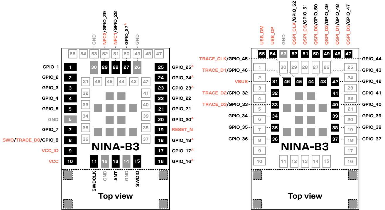
Figure 3: NINA-B30 series pin assignment (top view)
