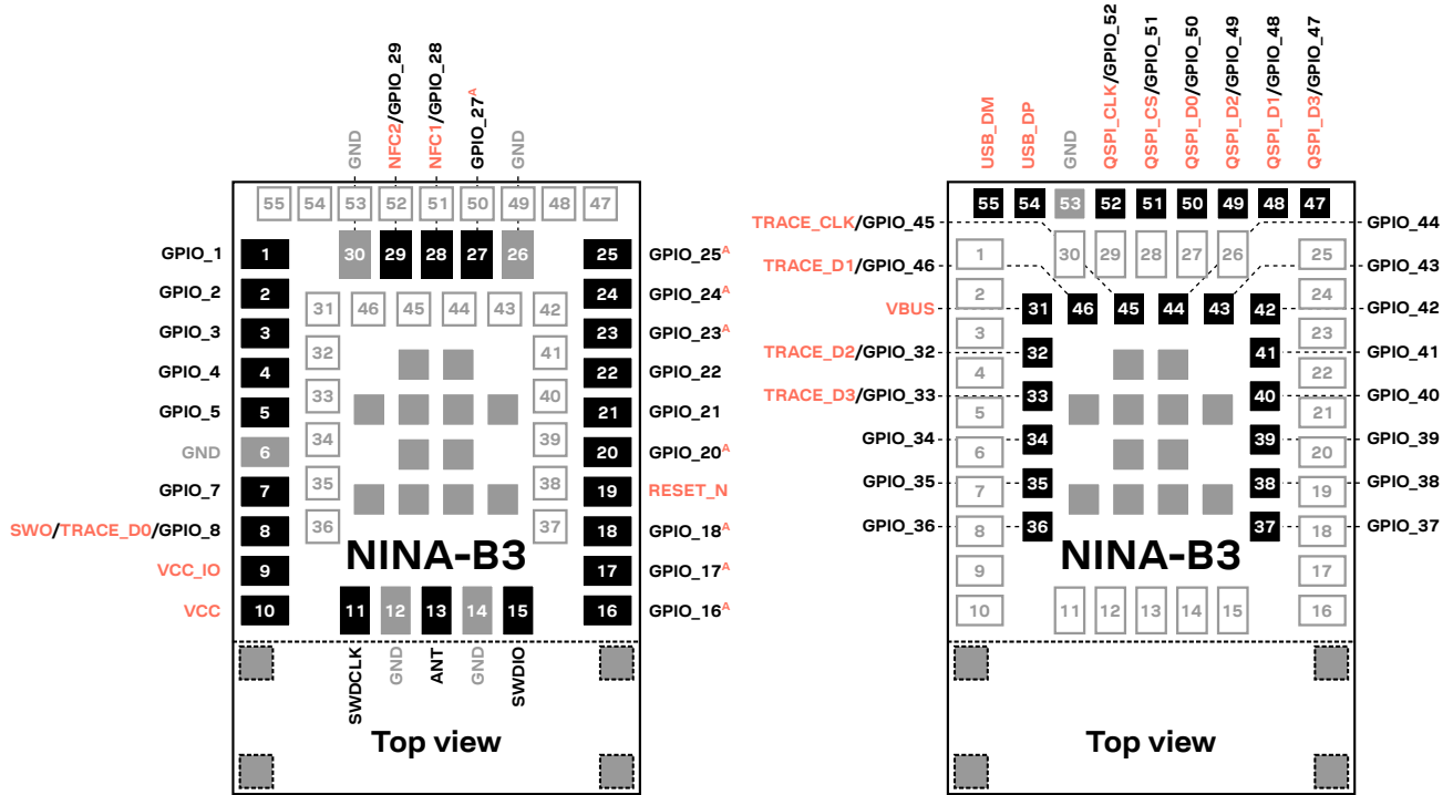
Figure 4: NINA-B30 series pin assignment (top view)
