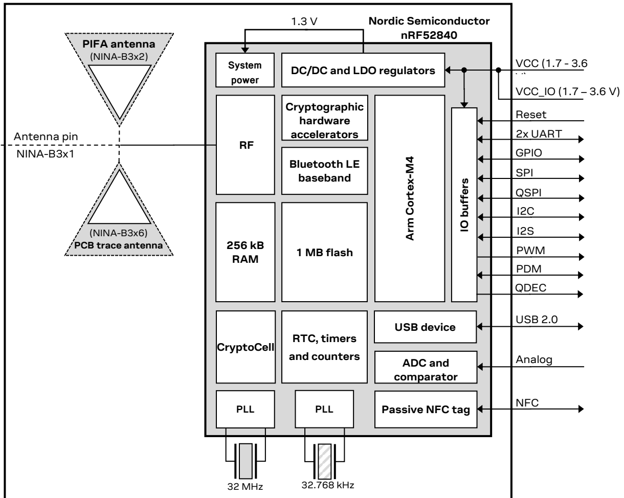
Figure 1: Block diagram of NINA-B3 series. 32.768 kHz crystal is not included in NINA-B306-01B
