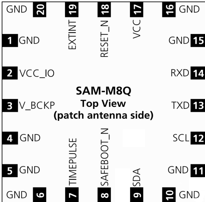
Figure 2: Pin assignment
