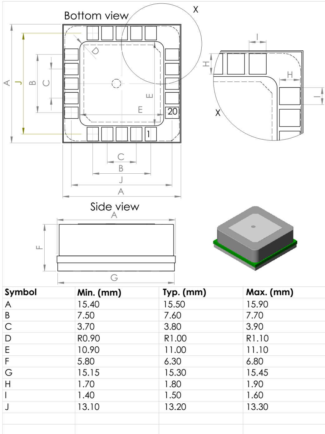
Figure 3: Dimensions
