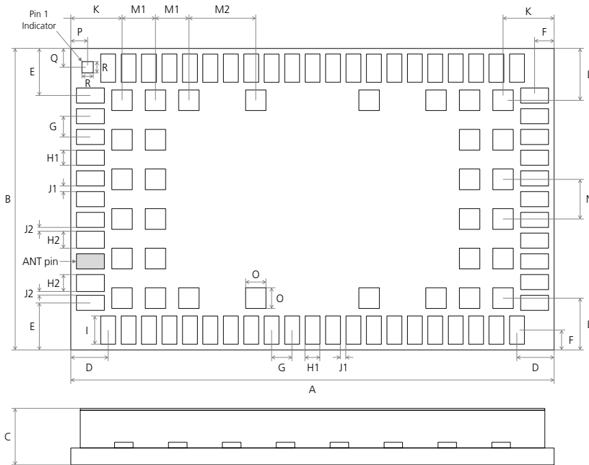
Figure 3: SARA-R4 series dimensions (bottom and side views)
