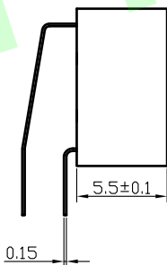
平推柄 short handle
