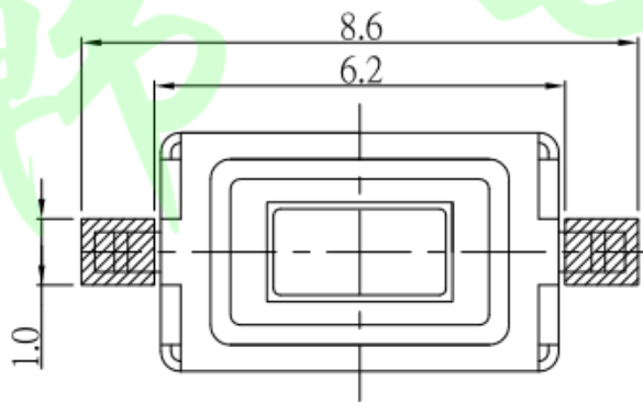
P.C.B MOUNTING PATTERN DIMENSION The following soldering patterns are recommended for reflow soldering
