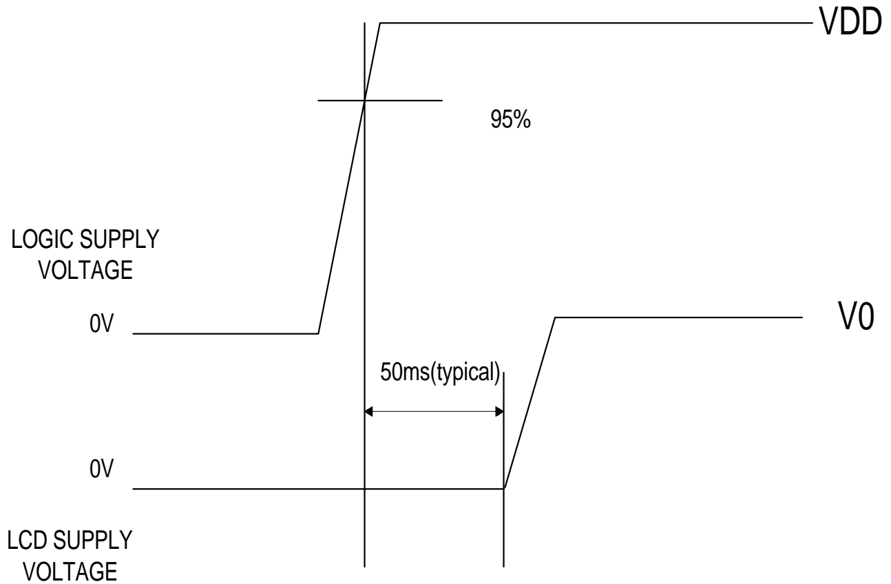
Figure 5: Timing diagram of VDD against V0.
