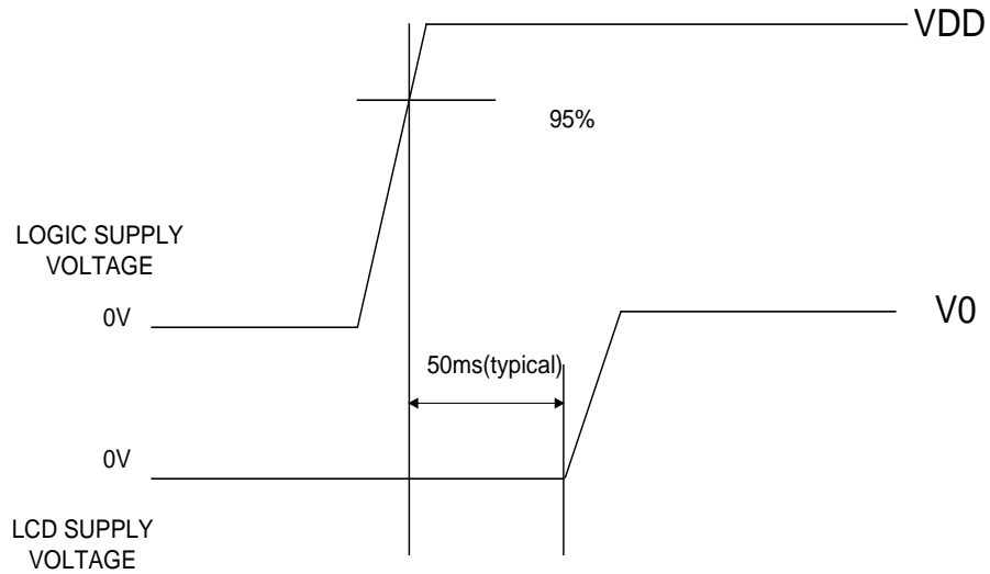
Figure 4: Timing Diagram of VDD Against V0.
