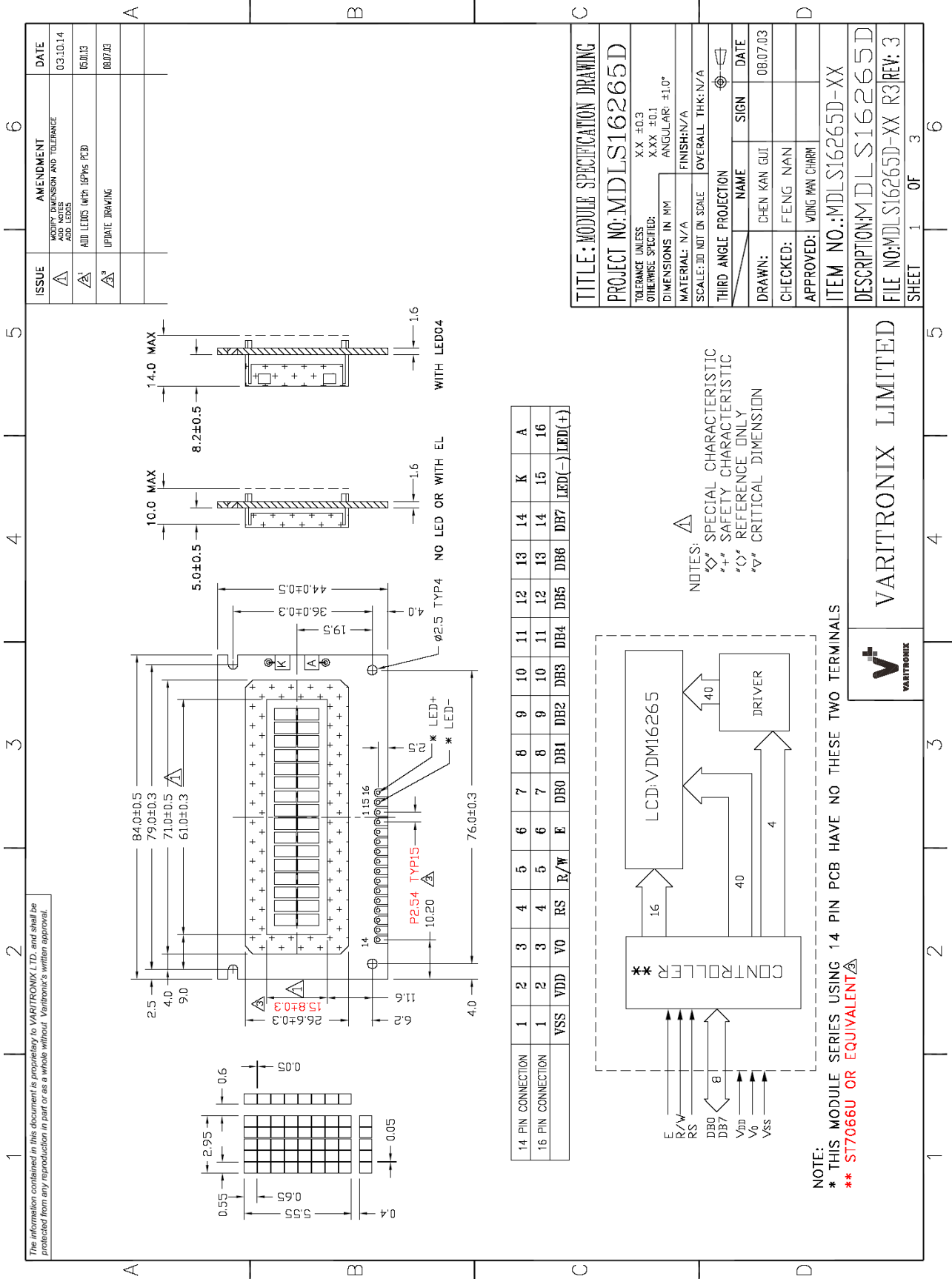
Figure 1: Module Specification
