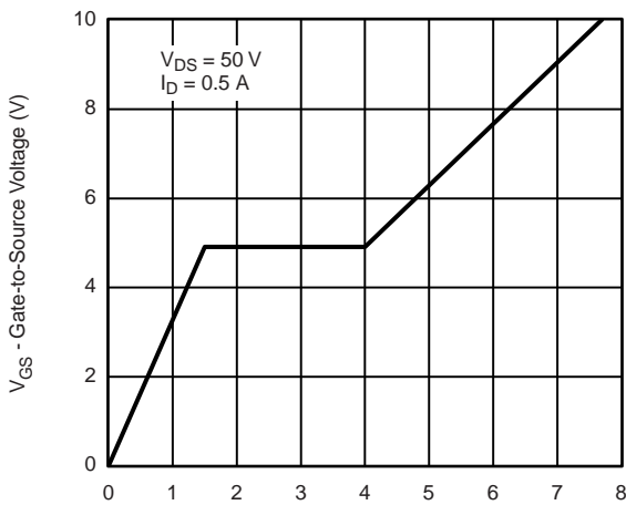
Q_g - Total Gate Charge (nC) Gate Charge
