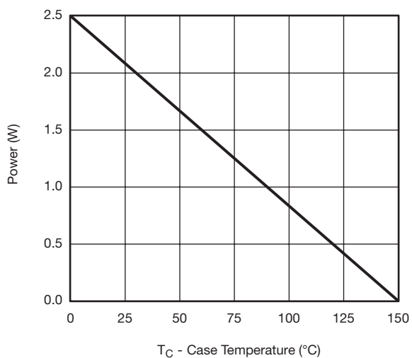
T_C - Case Temperature (°C) Power Derating, Junction-to-Foot
