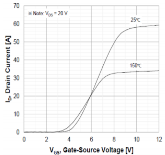
Transfer characteristics
