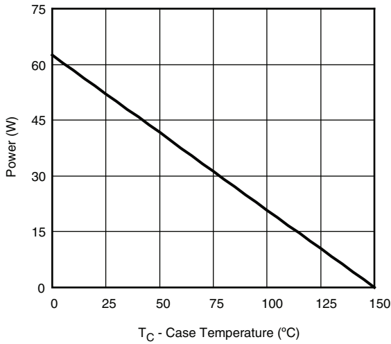
T_C - Case Temperature (°C) Power, Junction-to-Case
