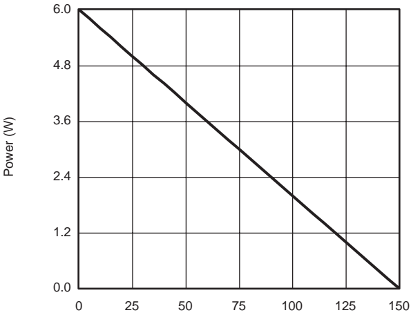
Power, Junction-to-Foot
