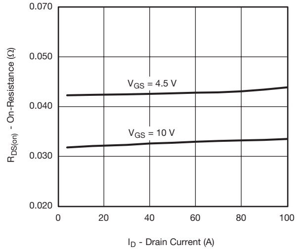
R_{DS(on)} - On-Resistance ( \Omega ) On-Resistance vs. Drain Current
