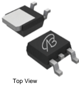
TO-252
