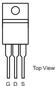
TO-220AB
