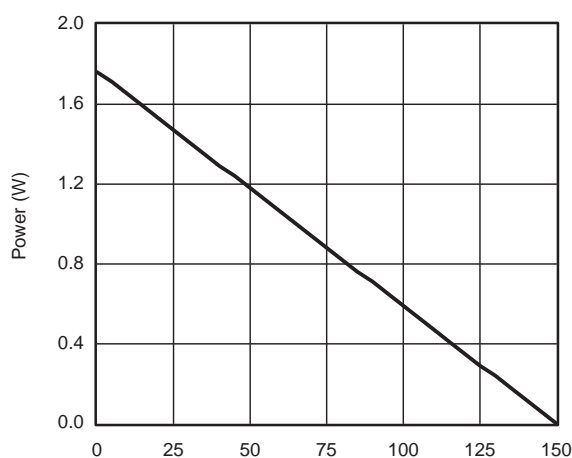
T A - Ambient Temperature (°C) Power Derating, Junction-to-Ambient
