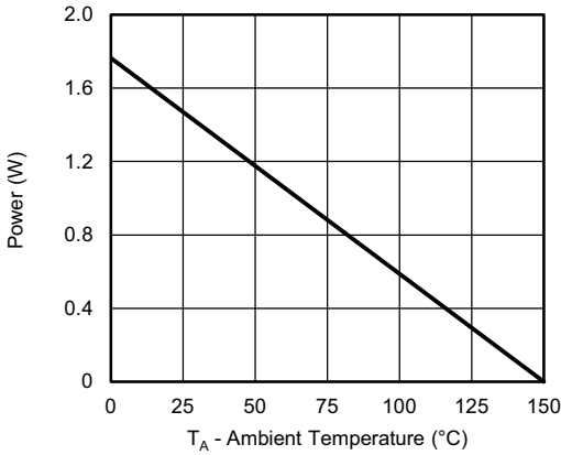
Power, Junction-to-Ambient
