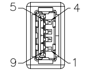
Conn.2
