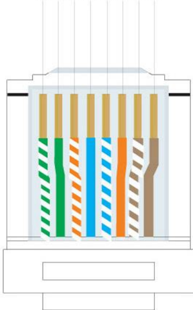
T568A standard
