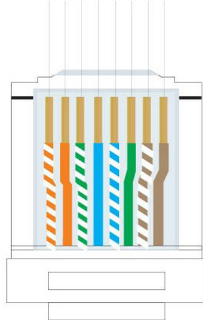
T568B standard
