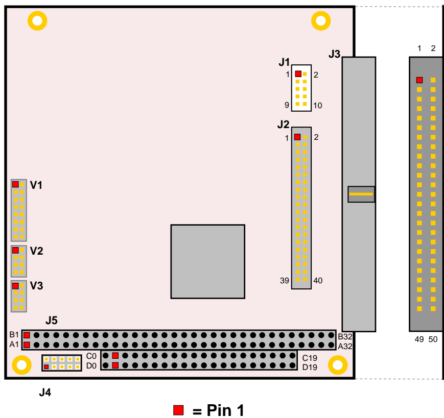
Figure 3. Connector Locations (Top) (Not to scale.)
