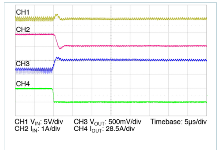
Figure 16 — 28.5A – 0A transient response: C_{IN} = 2.2\mu\text{F} , I_{IN} measured prior to C_{IN} , no external C_{OUT}
