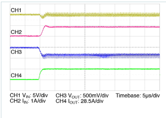
Figure 15 — 0A – 28.5A transient response: C_{IN} = 2.2\mu\text{F} , I_{IN} measured prior to C_{IN} , no external C_{OUT}
