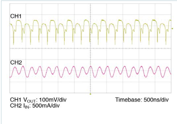
Figure 13 — Full load ripple, 2.2\mu\text{F} C_{IN} ; No external C_{OUT} , Board mounted module, scope setting : 20MHz analog BW
