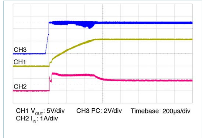
Figure 14 — Start up from application of PC; V_{IN} pre-applied C_{OUT} = 1200\mu\text{F}
