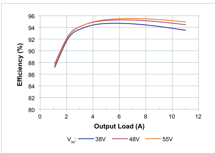
Figure 6 — Efficiency at T_{CASE} = 25^{\circ}C
