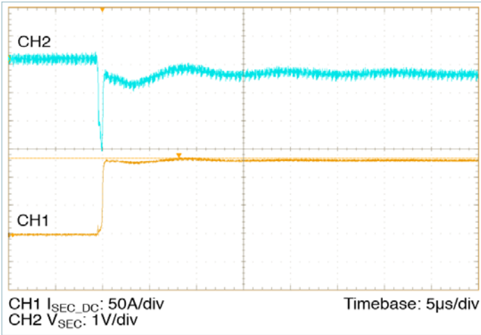
Figure 15 — 0 – 130A transient response: C_{PRI\_IN\_EXT} = 2700\mu F , no external C_{SEC\_OUT\_EXT}
