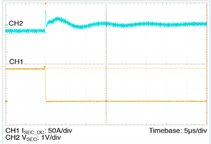
Figure 16 — 130 – 0A transient response: C_{PRI\_IN\_EXT} = 2700\mu F , no external C_{SEC\_OUT\_EXT}
