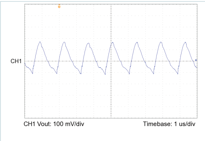
Figure 17 — Output voltage ripple, V_{IN} = 48\text{ V} , V_{OUT} = 24.0\text{ V} , C_{OUT\_EXT} = 1000\ \mu\text{F} , R_{LOAD} = 1.800\ \Omega
