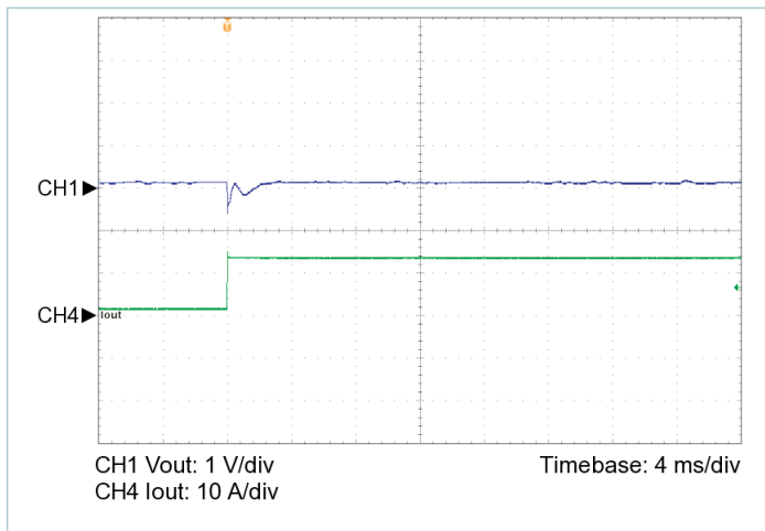
Figure 6 — 10% to 100% load transient response, V_{IN} = 48\text{ V} , nominal trim, C_{OUT\_EXT} = 1000\ \mu\text{F}
