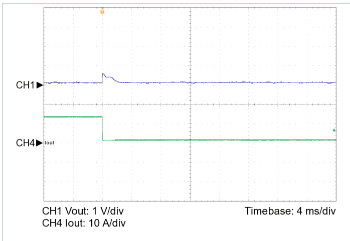
Figure 5 — 100% to 10% load transient response, V_{IN} = 48\text{ V} , nominal trim, C_{OUT\_EXT} = 1000\ \mu\text{F}
