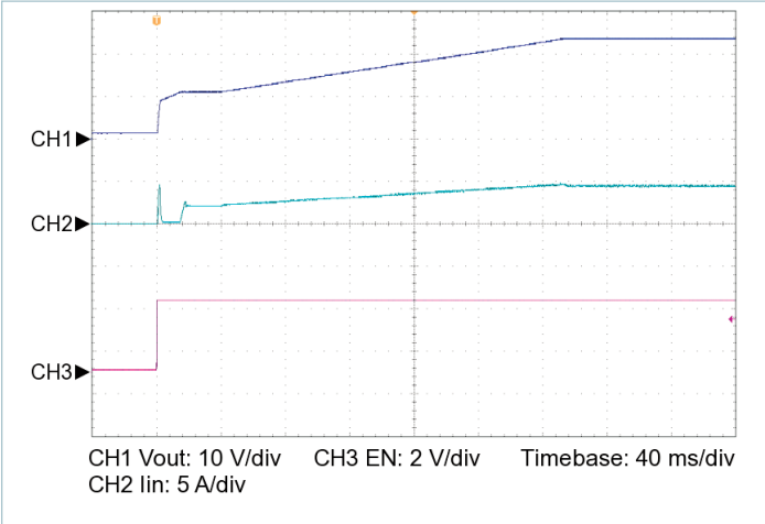
Figure 15 — Startup from EN, V_{IN} = 48\text{ V} , C_{OUT\_EXT} = 10000\ \mu\text{F} , R_{LOAD} = 1.800\ \Omega
