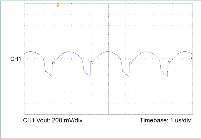
Figure 16 — Output voltage ripple, V_{IN} = 28\text{ V} , V_{OUT} = 3.3\text{ V} , C_{OUT\_EXT} = 1000\ \mu\text{F} , R_{LOAD} = 0.091\ \Omega
