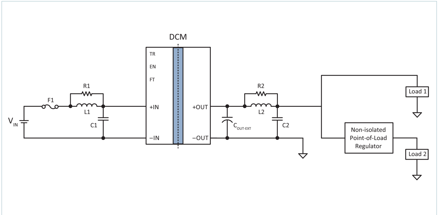
Typical Application 1: Single DCM3623x50M53C2y7z, to a non-isolated regulator, and direct to load
