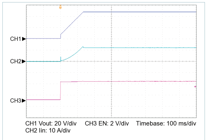
Figure 14 — Startup from EN, V_{IN} = 28\text{ V} , C_{OUT\_EXT} = 2000\ \mu\text{F} , R_{LOAD} = 7.200\ \Omega
