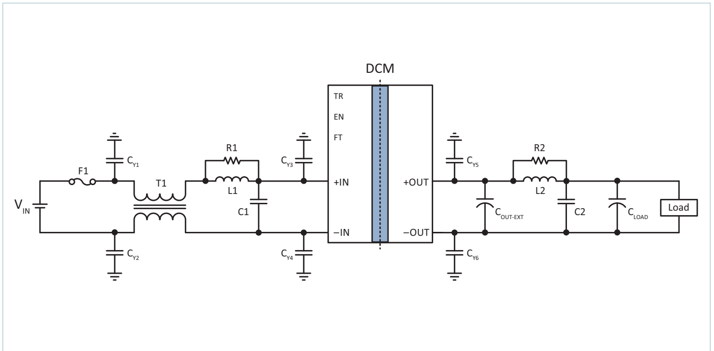
Typical Application 2: Single DCM3623x50M53C2y7z with common- and differential-mode input filters
