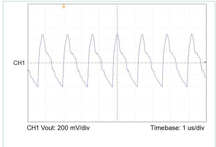
Figure 16 — Output voltage ripple, V_{IN} = 28\text{ V} , V_{OUT} = 48.0\text{ V} , C_{OUT\_EXT} = 200\ \mu\text{F} , R_{LOAD} = 7.200\ \Omega
