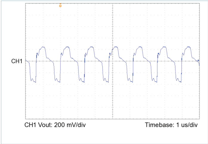
Figure 19 — Output voltage ripple, V_{IN} = 48\text{ V} , V_{OUT} = 15.0\text{ V} , C_{OUT\_EXT} = 1000\ \mu\text{F} , R_{LOAD} = 0.701\ \Omega
