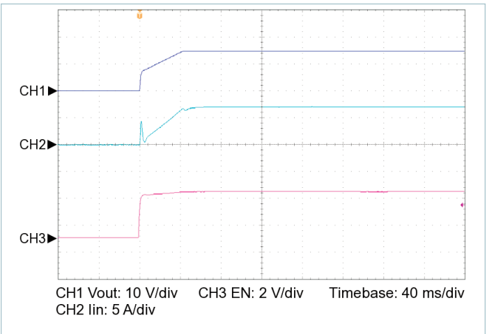
Figure 17 — Startup from EN, V_{IN} = 48\text{ V} , C_{OUT\_EXT} = 10000\ \mu\text{F} , R_{LOAD} = 0.701\ \Omega
