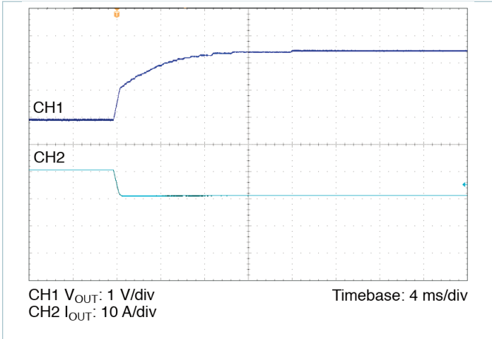
Figure 7 — 100% to 10% load transient response, V_{IN} = 300\text{ V} , nominal trim, C_{OUT\_EXT} = 220\ \mu\text{F}
