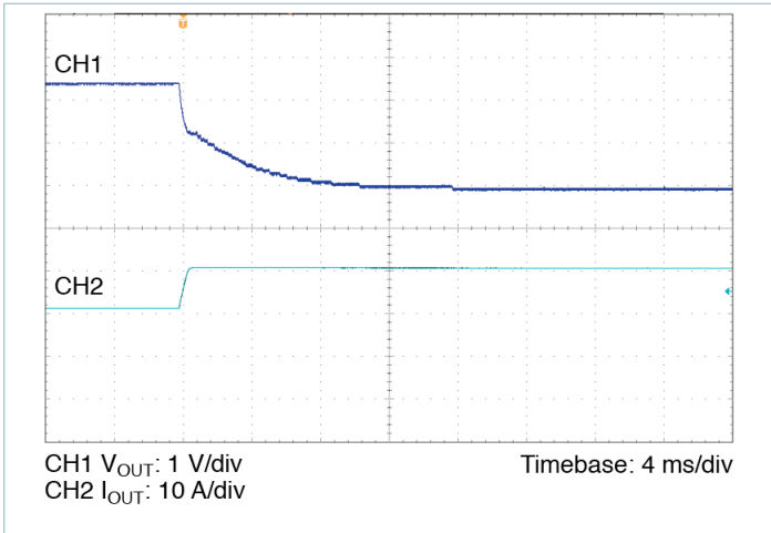
Figure 8 — 10% to 100% load transient response, V_{IN} = 300\text{ V} , nominal trim, C_{OUT\_EXT} = 220\ \mu\text{F}
