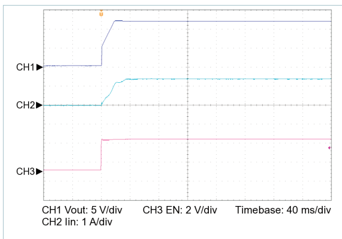
Figure 14 — Startup from EN, V_{IN} = 300\text{ V} , C_{OUT\_EXT} = 10000\ \mu\text{F} , R_{LOAD} = 0.359\ \Omega
