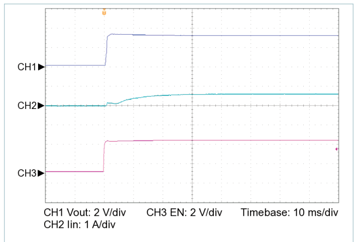
Figure 14 — Startup from EN, V_{IN} = 270\text{ V} , C_{OUT\_EXT} = 10000\ \mu\text{F} , R_{LOAD} = 0.073\ \Omega
