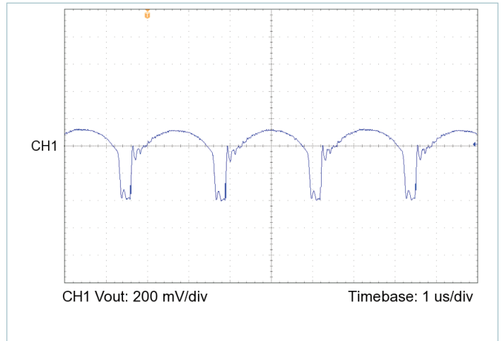
Figure 16 — Output voltage ripple, V_{IN} = 270\text{ V} , V_{OUT} = 3.3\text{ V} , C_{OUT\_EXT} = 1000\ \mu\text{F} , R_{LOAD} = 0.073\ \Omega
