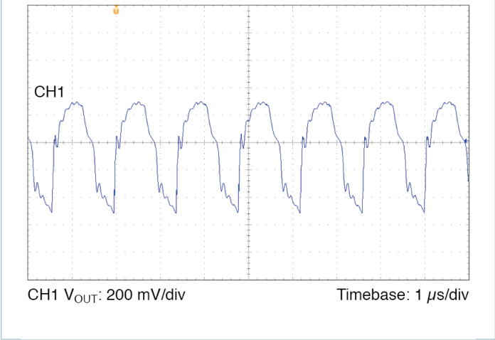
Figure 16 — Output voltage ripple, V_{IN} = 270\text{ V} , V_{OUT} = 28.0\text{ V} , C_{OUT\_EXT} = 200\text{ }\mu\text{F} , R_{LOAD} = 1.568\text{ }\Omega
