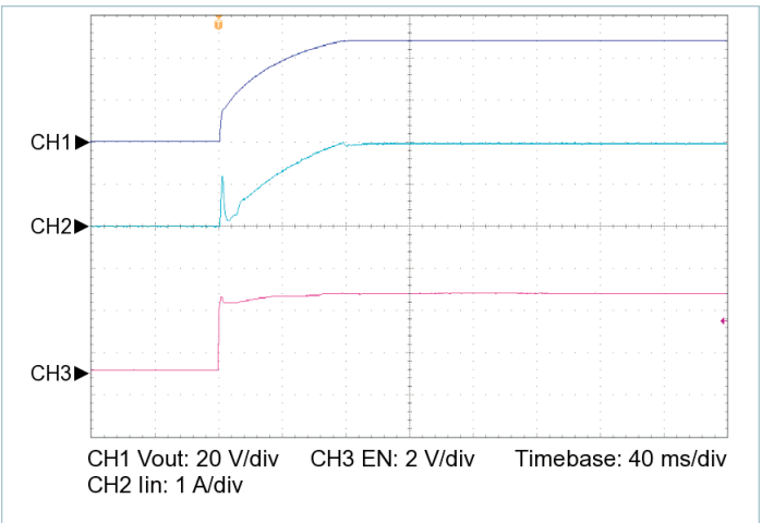
Figure 17 — Startup from EN, V_{IN} = 270\text{ V} , C_{OUT\_EXT} = 2200\text{ }\mu\text{F} , R_{LOAD} = 4.607\text{ }\Omega
