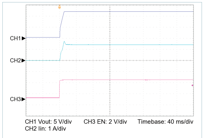
Figure 14 — Startup from EN, V_{IN} = 275\text{ V} , C_{OUT\_EXT} = 10000\ \mu\text{F} , R_{LOAD} = 0.383\ \Omega
