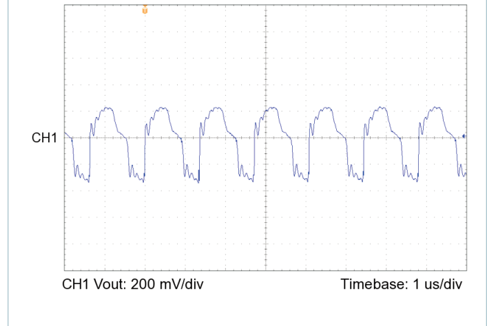
Figure 16 — Output voltage ripple, V_{IN} = 275\text{ V} , V_{OUT} = 15.0\text{ V} , C_{OUT\_EXT} = 1000\text{ }\mu\text{F} , R_{LOAD} = 0.600\text{ }\Omega
