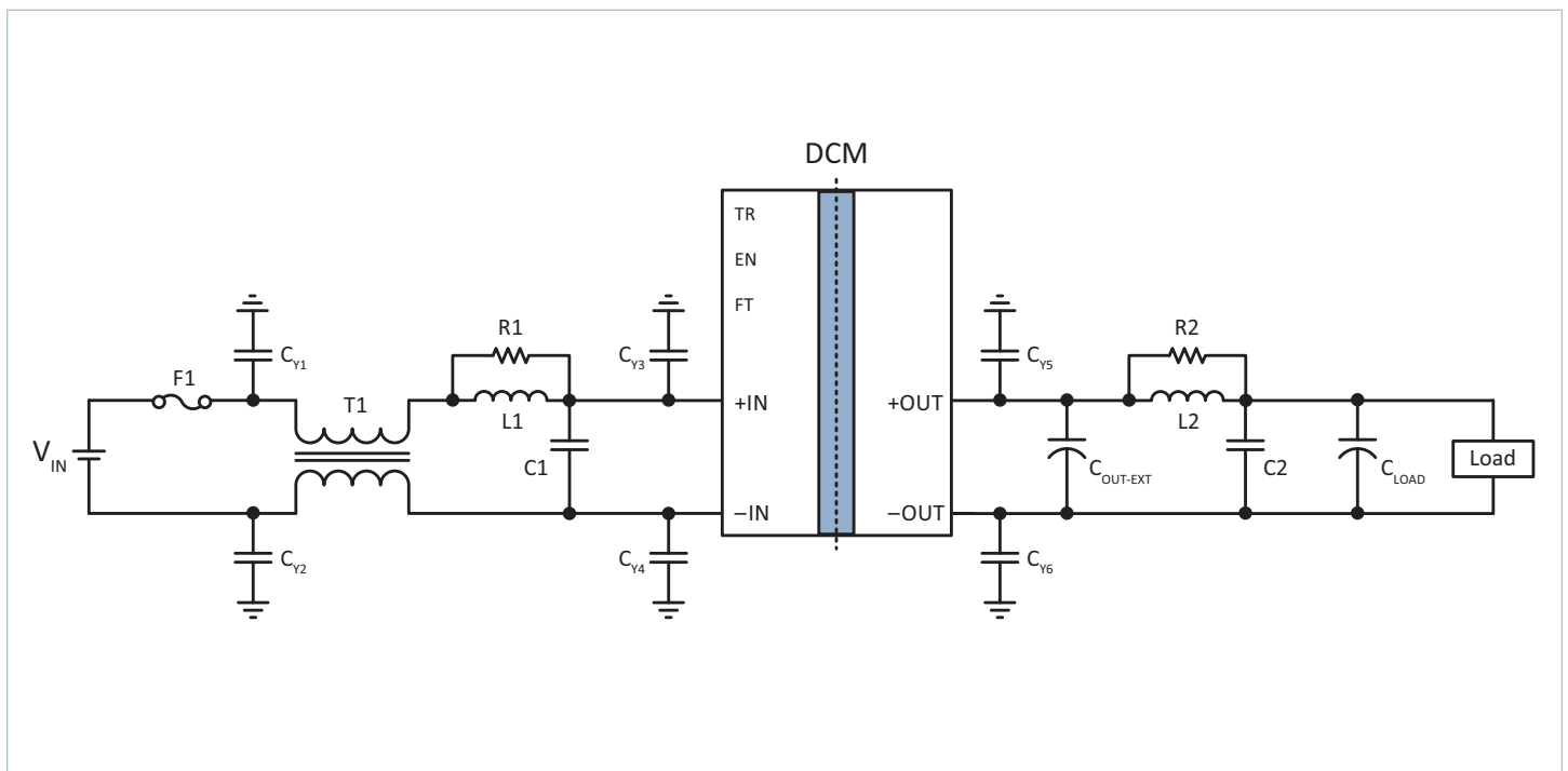
Typical Application 2: Single DCM4623xD2N17C8y7z with common- and differential-mode input filters
