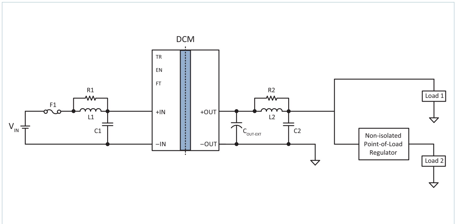
Typical Application 1: Single DCM4623xD2N17C8y7z, to a non-isolated regulator, and direct to load
