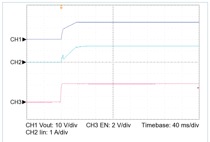
Figure 14 — Startup from EN, V_{IN} = 275\text{ V} , C_{OUT\_EXT} = 10000\ \mu\text{F} , R_{LOAD} = 0.600\ \Omega
