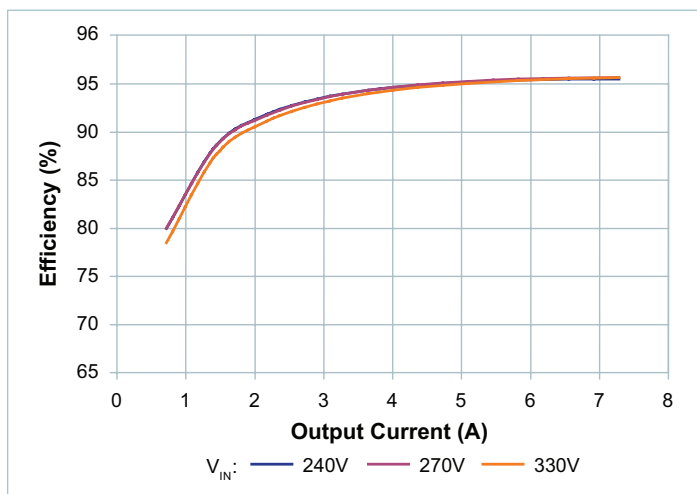
Figure 4 — Efficiency at T_{CASE} = -55^{\circ}C
