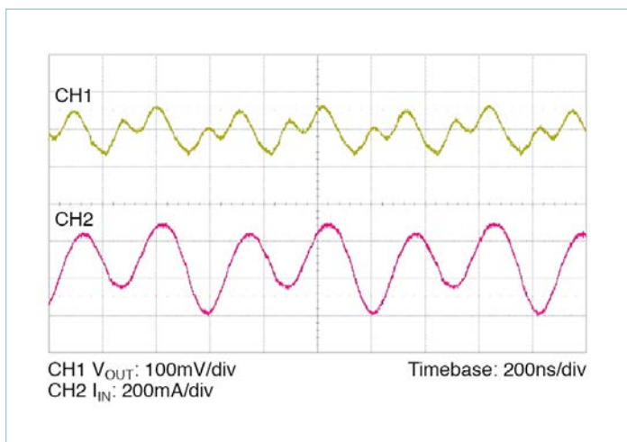
Figure 14 — Full load ripple, 100\mu F C_{IN} ; no external C_{OUT} . Board mounted module, scope setting: 20MHz analog BW
