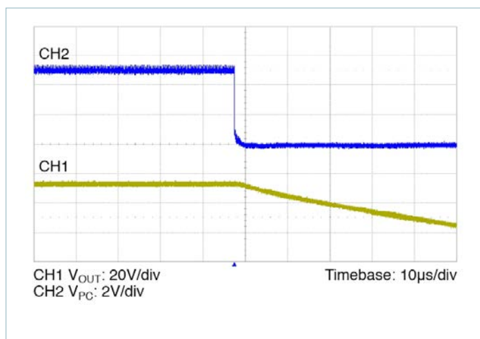
Figure 17 — PC disable waveform, 270V_{IN} , 100\mu F C_{OUT} full load
