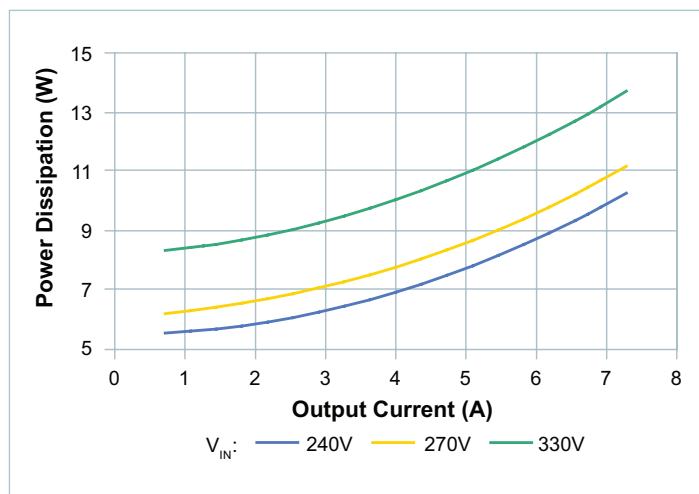
Figure 5 — Power dissipation at T_{CASE} = -55^{\circ}C
