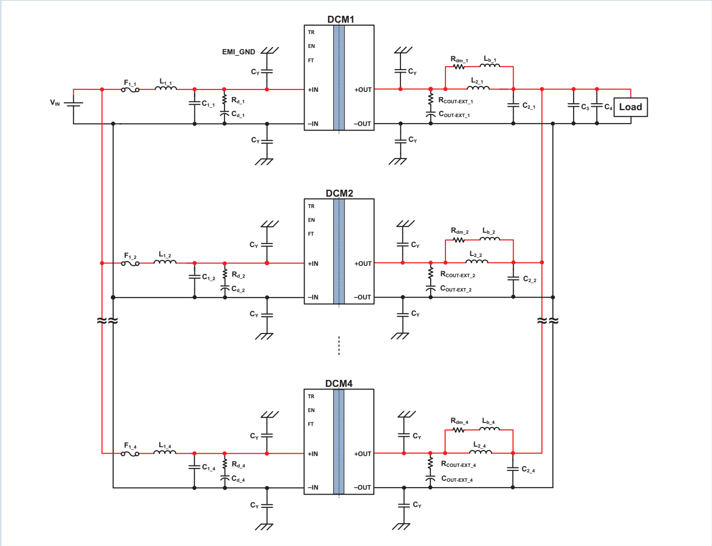
Typical Application 1: DCM4623xD2K06B5yzz in an array of four units
