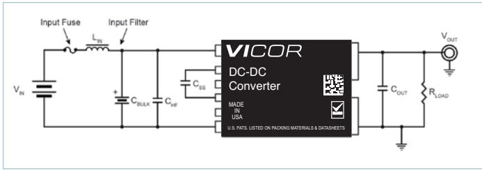
Figure 21 — PI31xx-01-HVIZ shown with system fuse, filter, decoupling and extended soft start
