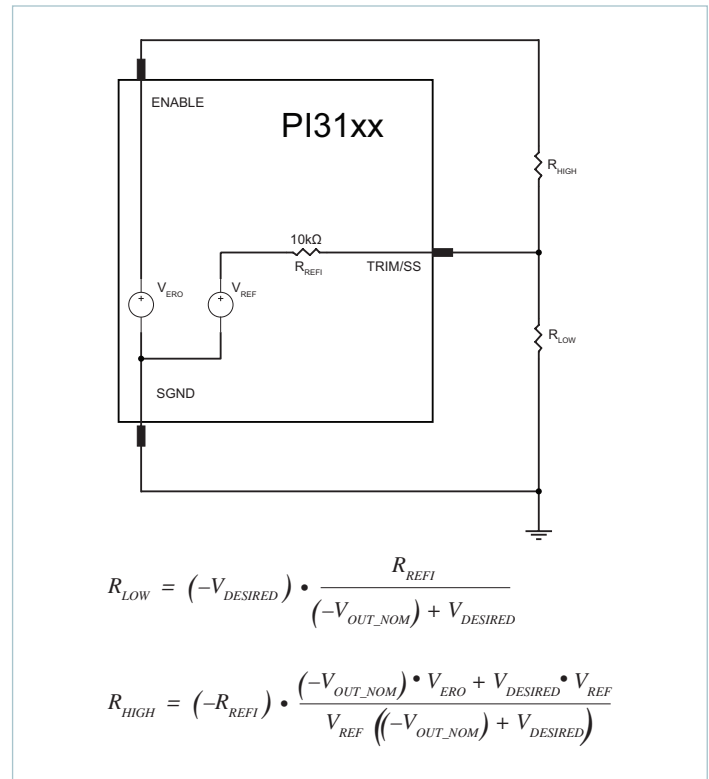
Figure 22 — Trim equations and equivalent circuit
