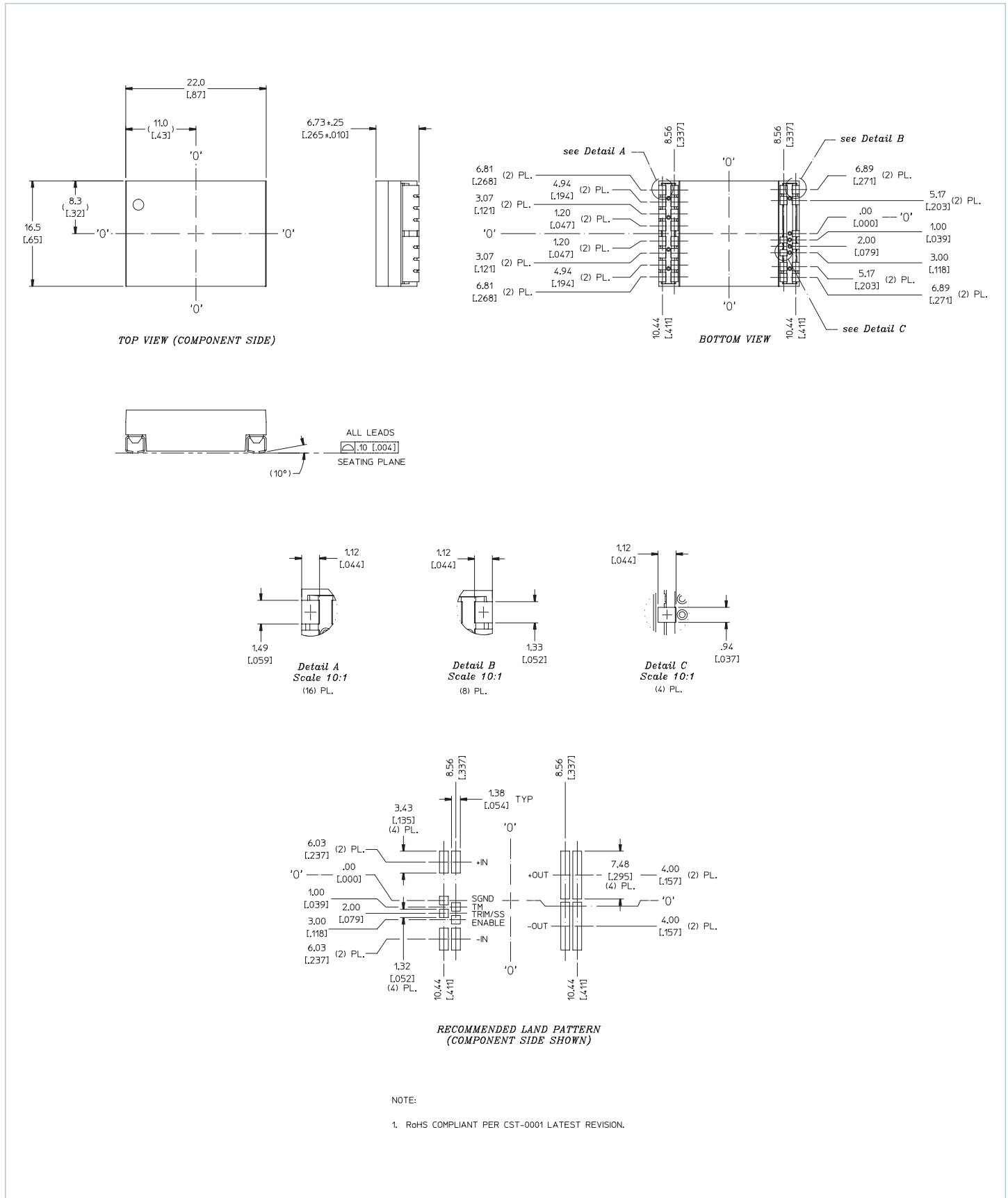
Figure 23 — Package outline & recommended PCB land pattern
